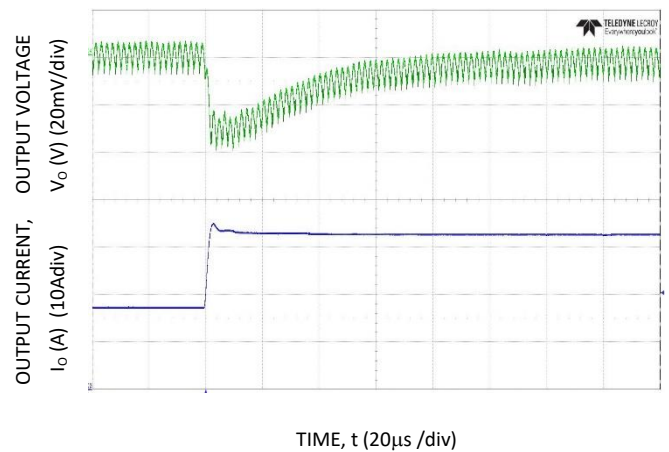
Figure 16. Transient Response to Dynamic Load Change from 50% to 100% at 12Vin, Cout=8x47uF+7x330uF, CTune=4.7nF, RTune=221Ω
