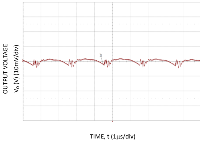
Figure 3. Typical output ripple ( C_0=8 \times 47 \mu\text{F} ceramic, V_{IN} = 12\text{V} , I_o = I_{o,max} ).
