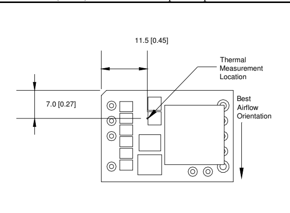
i6A24014A033V thermal measurement location – top view
