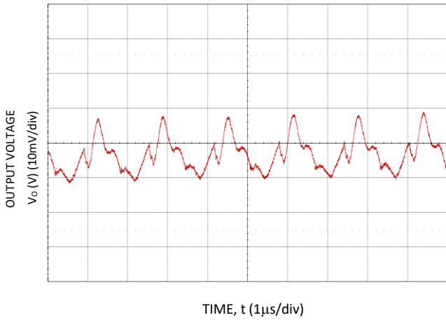
Figure 33. Typical output ripple and noise (Co=88µF ceramic, VIN = 12V, Io = Io,max.).
