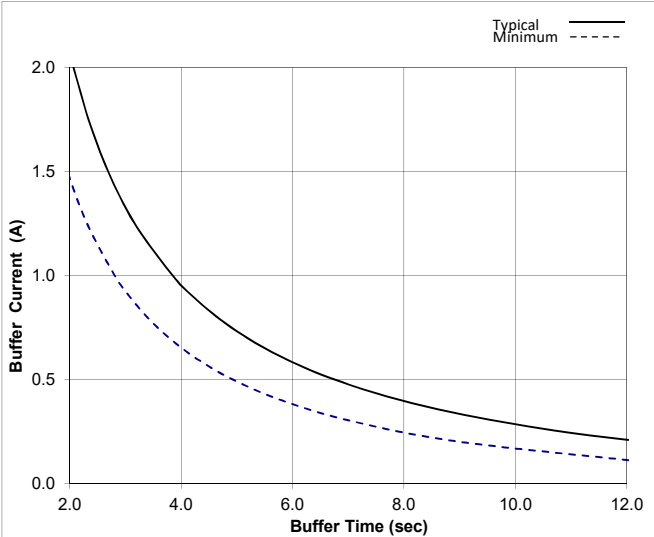
b) Buffer time for small buffer current : 2 - 12 sec
