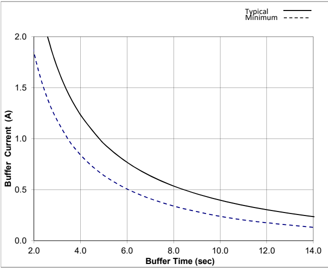
b) Buffer time for small buffer current : 2 - 14 sec
