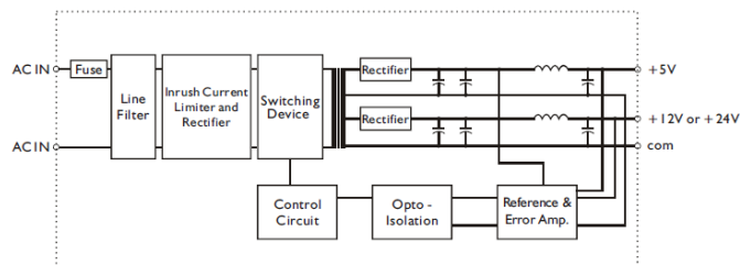
Block diagram for PA40A512D_01
