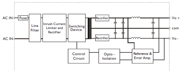
Block diagram for dual output
