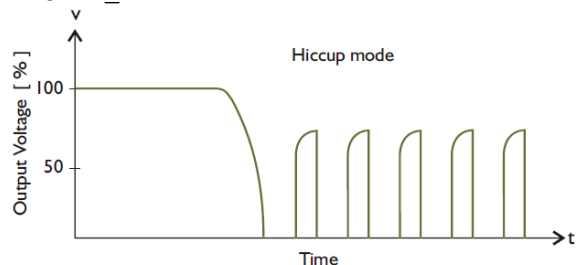
Typ. Current Limited Curve PA40A24_1
