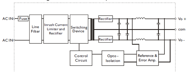
Block diagram for dual output
