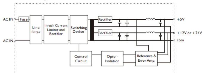
• Block diagram
